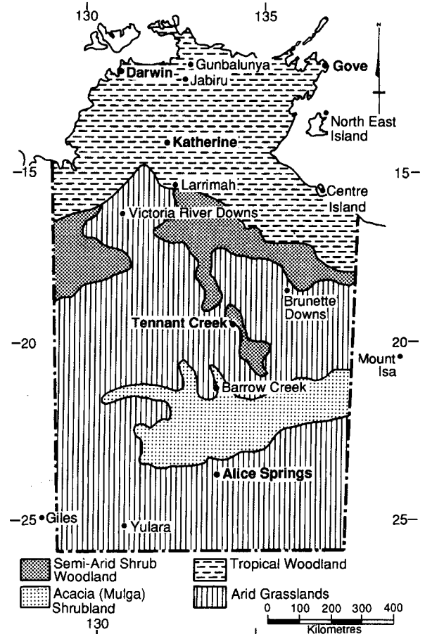
Figure 2. Major vegetation units in the NT (After Tapper et al. 1993).
