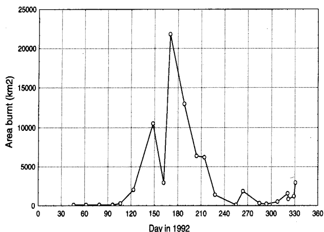
Figure 5. Graph of area burnt in km 2 between images.
